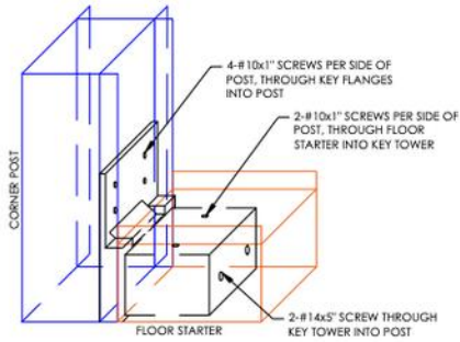
CORNER POST TO FLOOR CONNECTION
