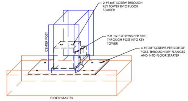
CENTER POST TO FLOOR CONNECTION
