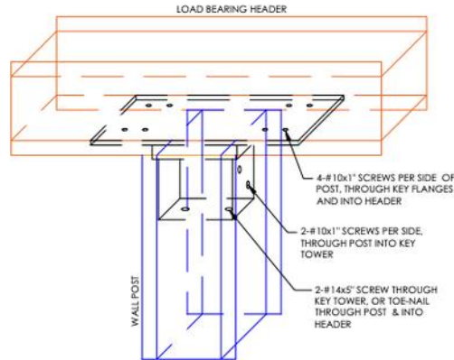
CENTER POST & HEADER CONNECTION
