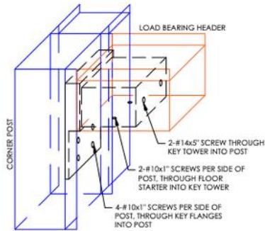
CORNER & HEADER CONNECTION
