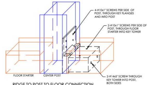
RIDGE TO POST TO FLOOR CONNECTION
