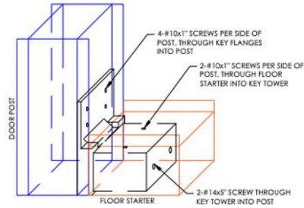
DOOR POST TO FLOOR CONNECTION
